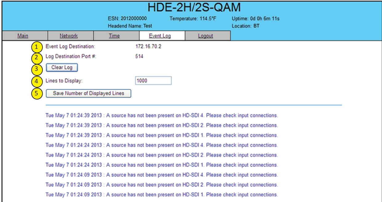
Figure 5.13 - "Event Log" Screen
