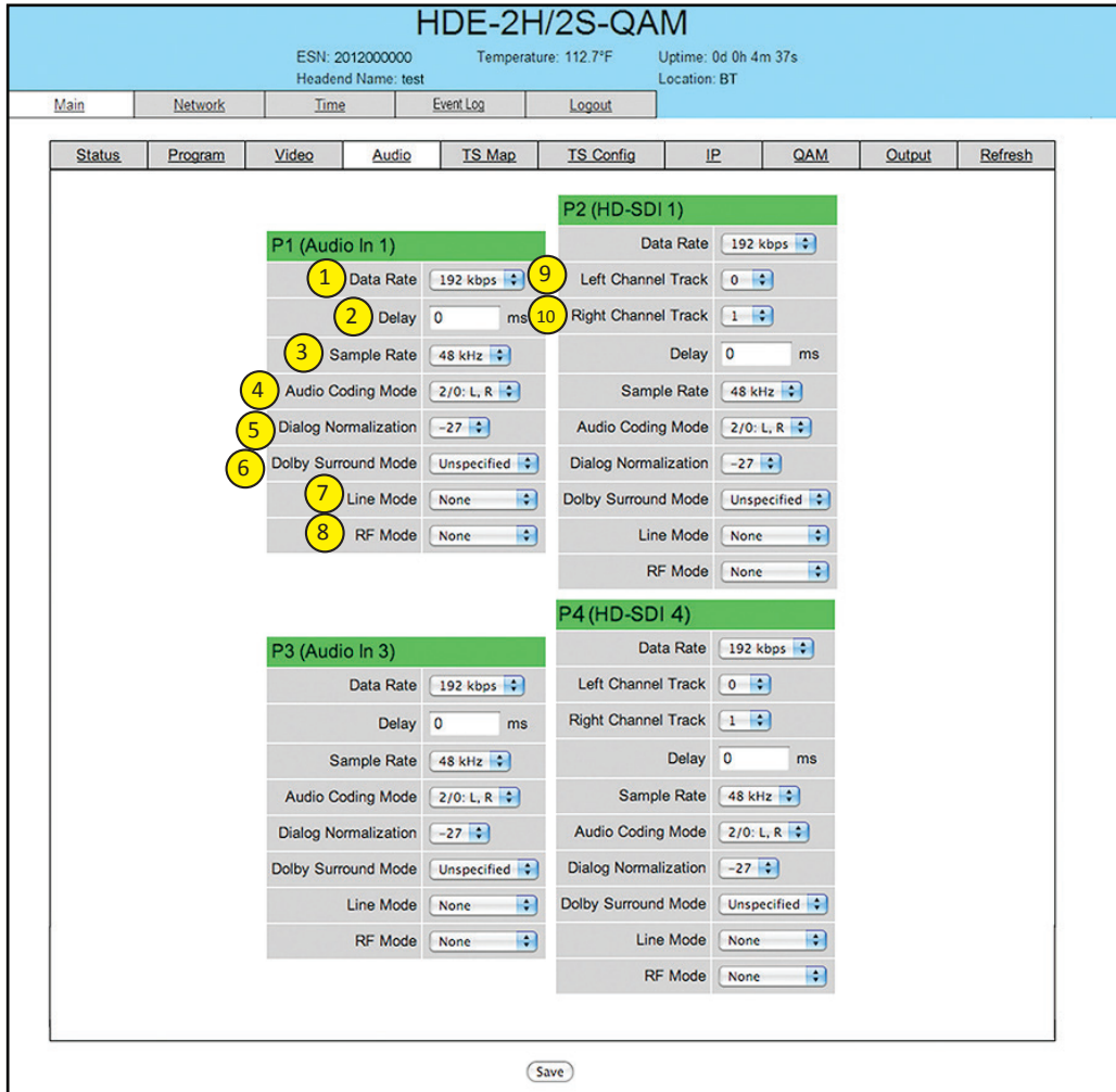
Figure 5.5 - "Main > Audio" Screen
