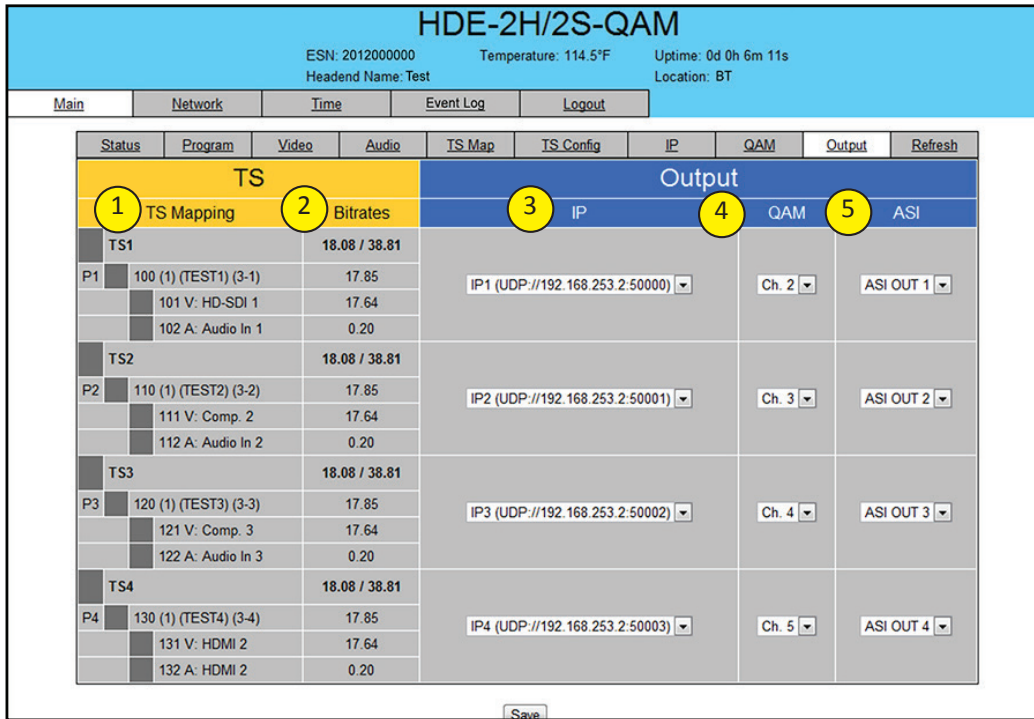
Figure 5.10 - "Main > Output" Screen
